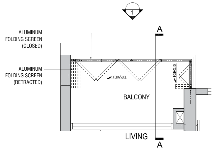
TYPICAL PLAN OF BALCONY / PES SCREEN
